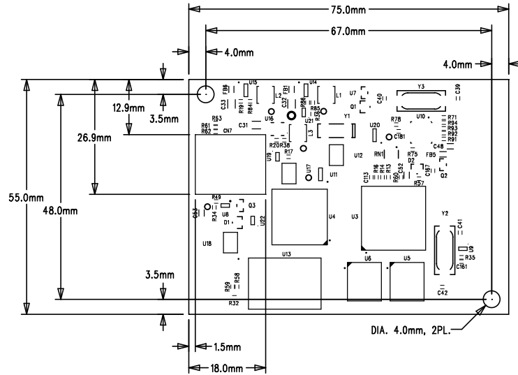
Connector Placement Top View
