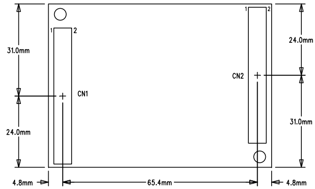
Connector Placement Top View
