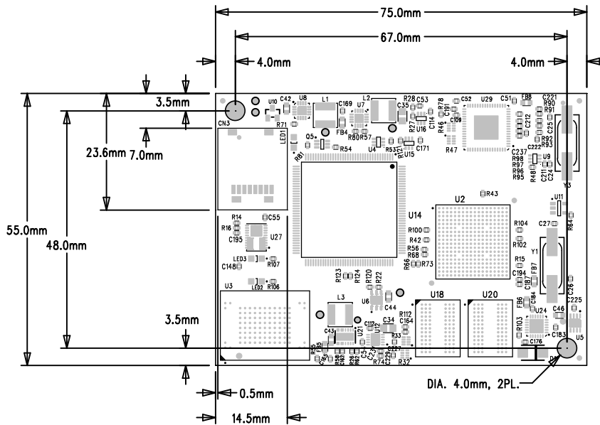
Connector Placement Top View
